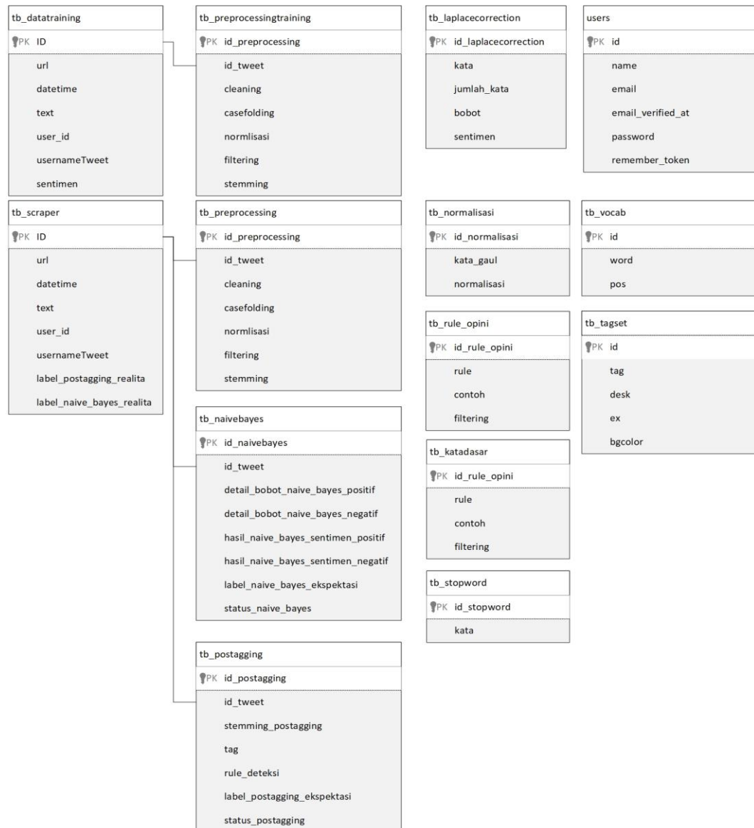
Gambar 5.1 Implementasi Database.
