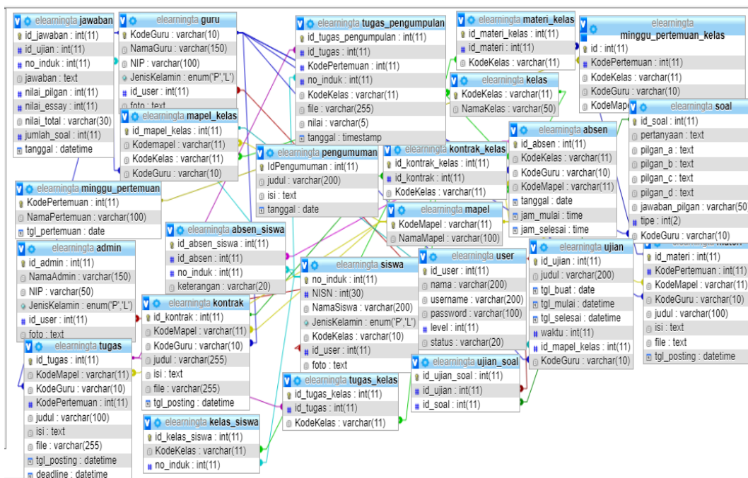
Gambar 4.1 Desain Basis Data
